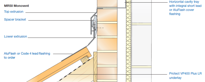
Fixing position of MR50 Monovent varies according to roof pitch
